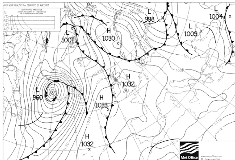
Fig 5 Synoptic Chart for Atlantic/Europe 20 th March 2003 (Source: Meteorological Office, Bracknell; www.wetter-zentrale.de )
