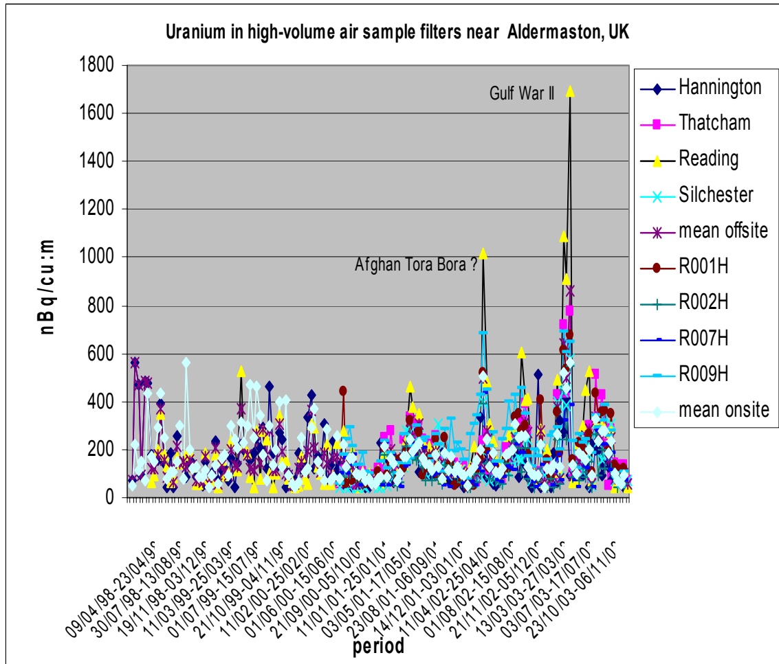
Fig 2 Uranium in air ( \text{nBq/m}^3 ) as shown by HVAS data points (*mostly) at two week intervals from 1998 near the Atomic Weapons Establishment, Aldermaston at four offsite and four onsite positions, R001, R002, R007 and R009. The two major excursions are labelled Gulf War 2 and Afghan Tora Bora. (* before 2000 measurements were taken at longer intervals).
