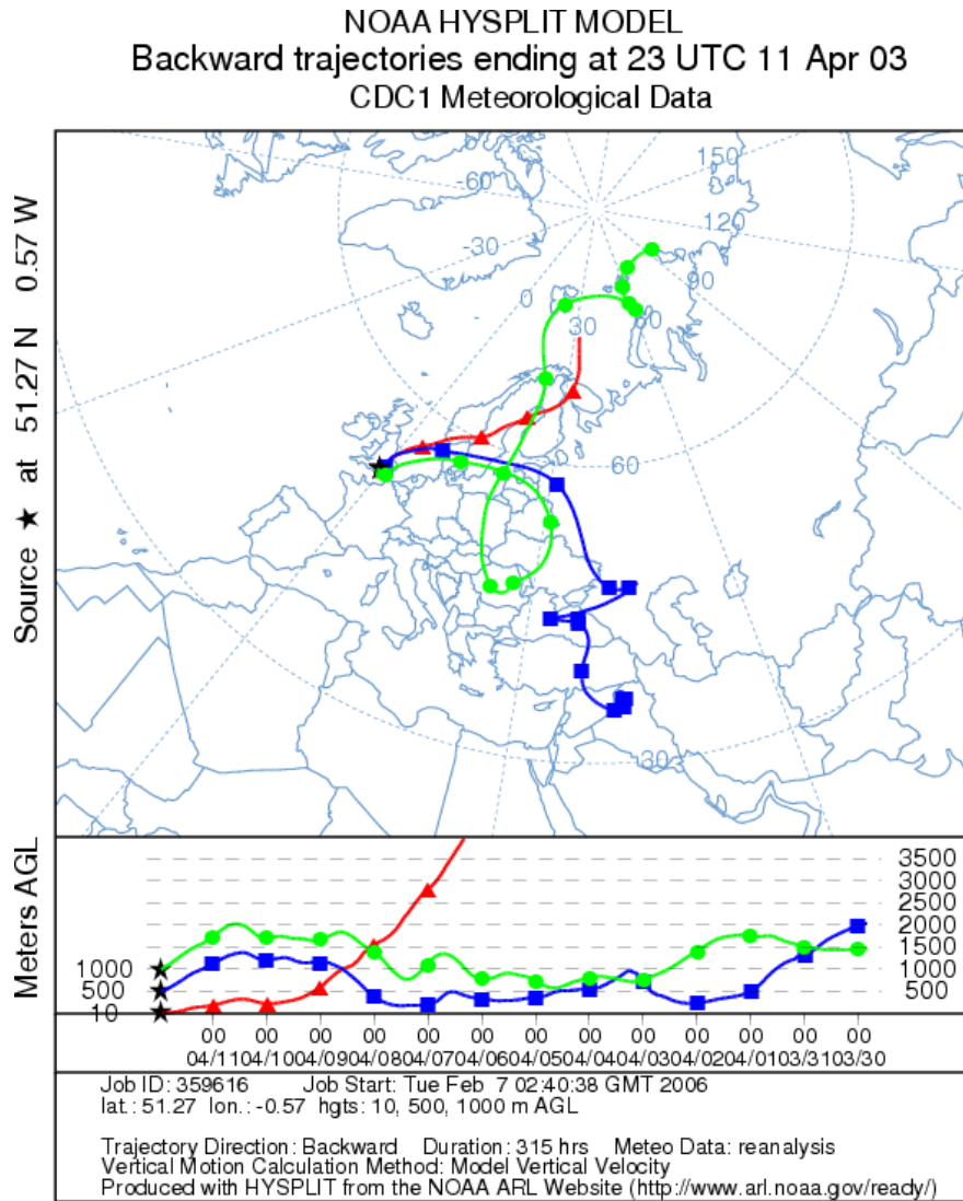
Fig 8 NOAA HYSPLIT calculated backward trajectory for sources of air at various levels (10, 500 and 1000m at Reading) arriving in Reading on 11 th April 2003. Each point represents 24 hrs .
