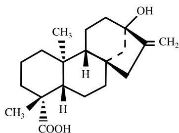
Steviol (C 20 H 30 O 3 )
