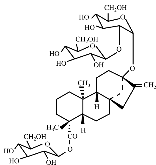
Stevioside (C 38 H 60 O 18 )
